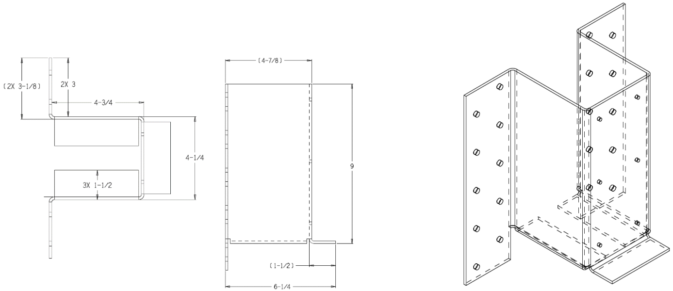
FIGURE 1 – MTWDeck Bracket
