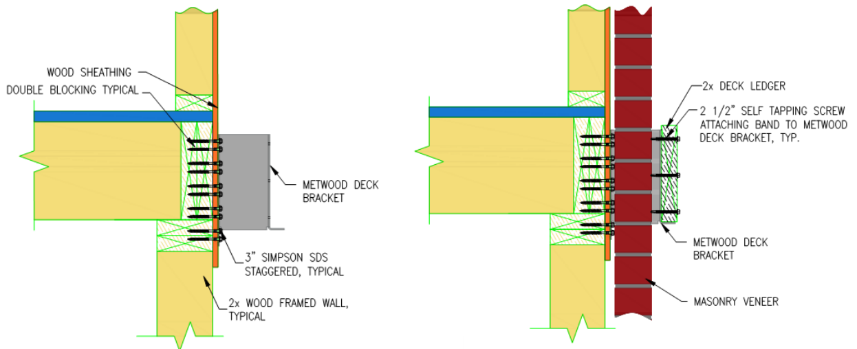
FIGURE 2 – Installation Diagram
